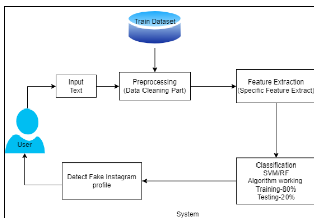
Fig.System Architecture
